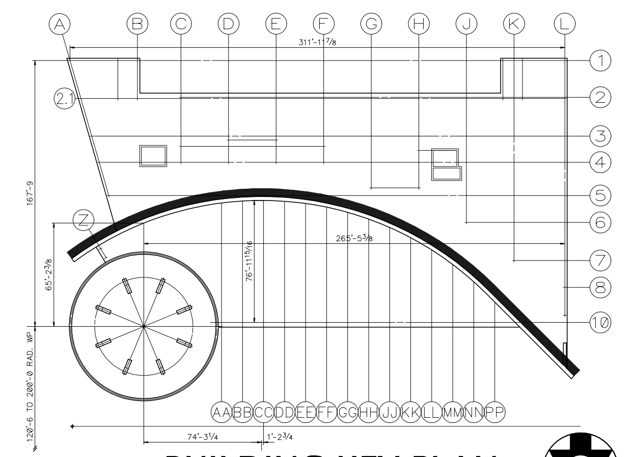
BUILDING KEY PLAN
