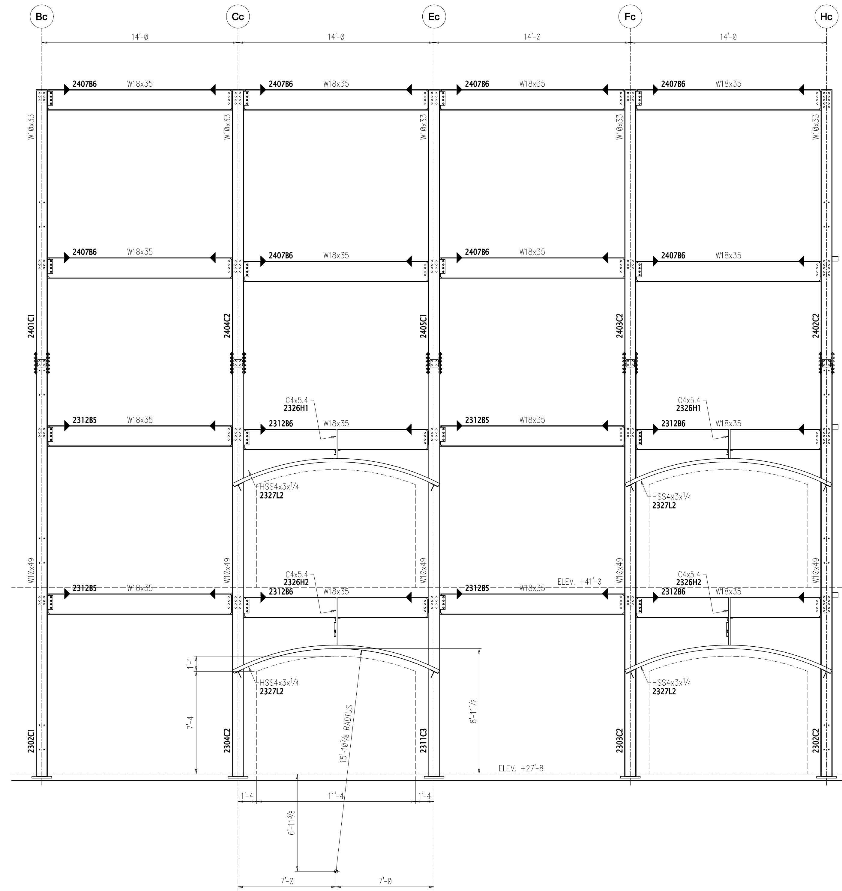
1 ELEVATION ALONG COLUMN LINE 47 E2205 LOOKING WEST
